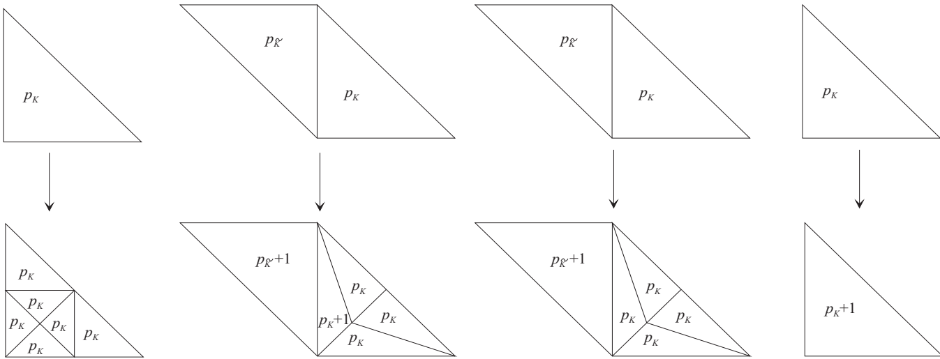
Figure 2: Definition of the polynomial degrees. From left to right: Pic1: regular refinement. Pic 2: K is h -refined, \tilde{K} is p -refined and p_{\tilde{K}} \geq p_K . Pic 3: K is h -refined, \tilde{K} is p -refined and p_{\tilde{K}} < p_K . Pic 4: p -refinement.
