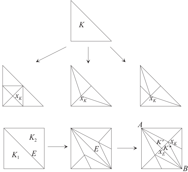
Figure 1: Refinement patterns of a triangle which satisfies the interior node property. Second row, from left to right: Pic. 1: Regular refinement. Pic. 2,3: Refinement patterns for the elimination of hanging nodes. Third row: If two triangles K_1, K_2 share an edge E and they will be both h -refined, then the common edge E must get an interior point x_E .
